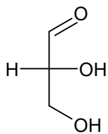
glyceraldehyd
